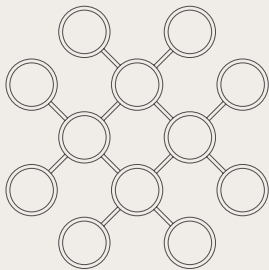
LIILA 12 Dimensions 845mm x 845mm x 170mm Glass dimensions ø140mm Options nordic gold / opal or nordic gold / optic clear Light source G9
