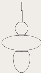
RIZZATTO 43 Dimensions ø400mm x 626mm Options satin brass / opal or satin silver / opal Cable colour gold or silver fabric Cable Length max 4000mm Light source E27
